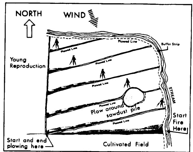
Figure 10-7. Backfire technique.
